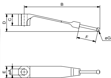
Hold-down spring with ball point
